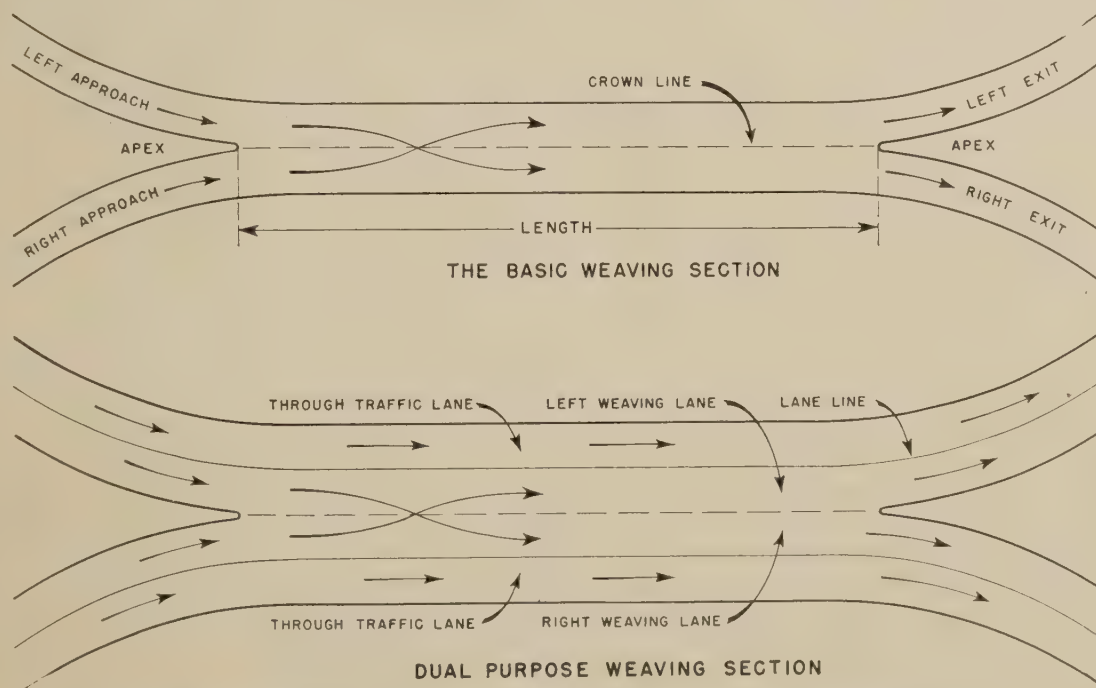
Figure 37 (above).—The basic weaving section: all traffic weaves.
